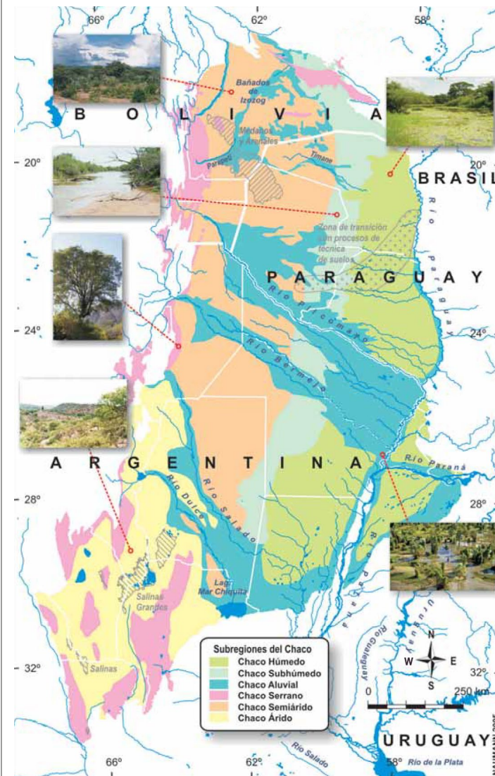
MAP 3 | Ecozones in the Gran Chaco
