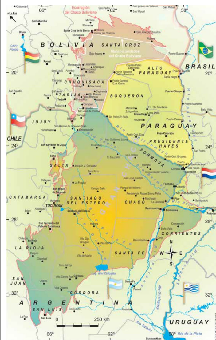
MAP 2 | Political organization of the Gran Chaco
